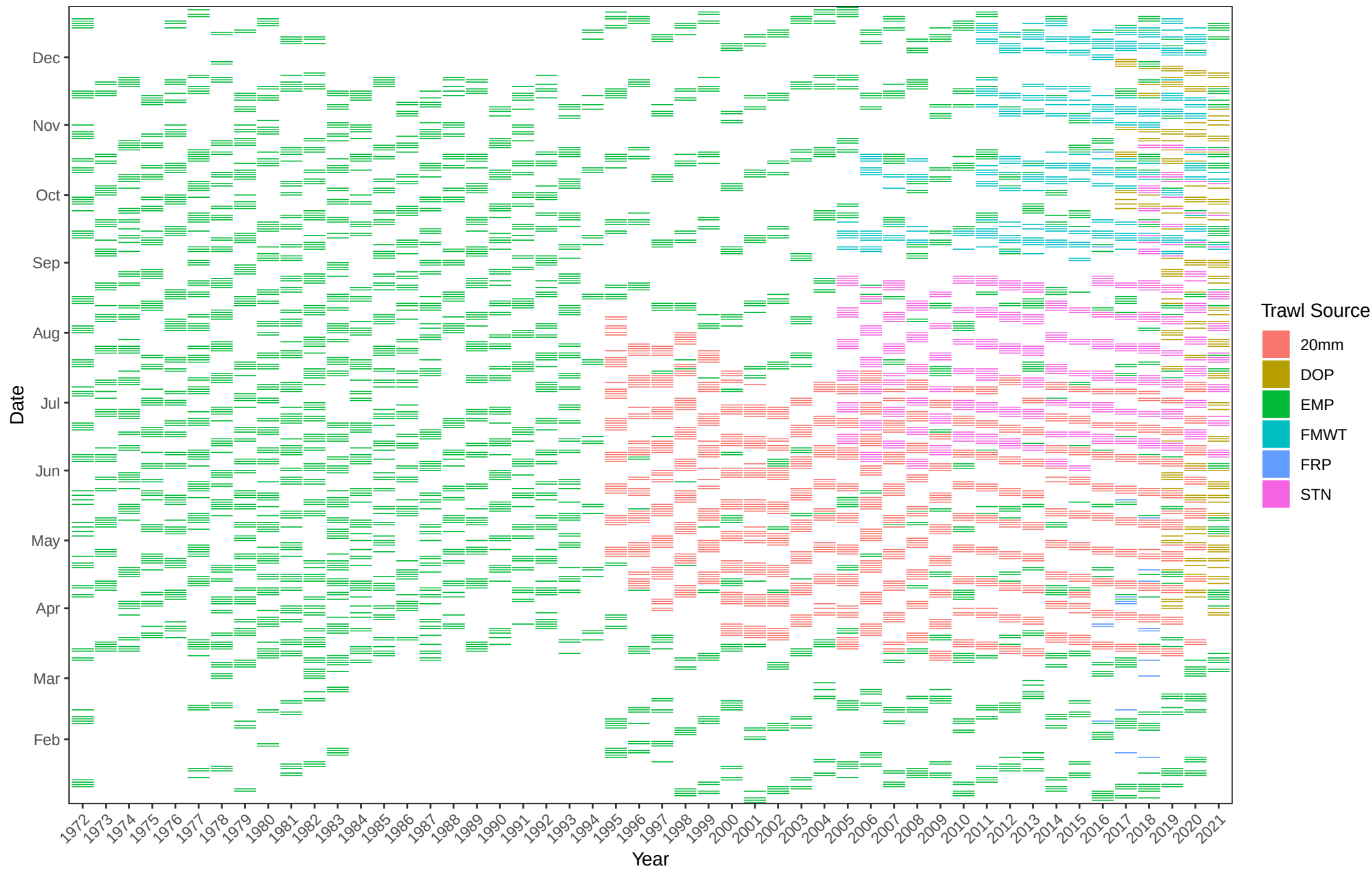
Sampling Dates by Year and Trawl Source
